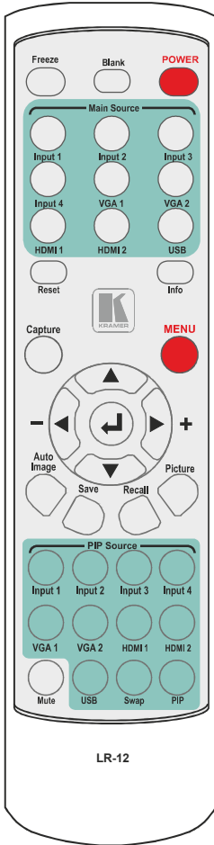
Figure 8: IR Remote Control Transmitter
