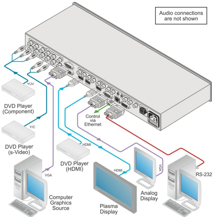
Figure 3: Connecting to the VP-729 Rear Panel
